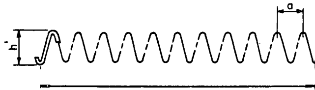
TYPICAL STIRRUP
